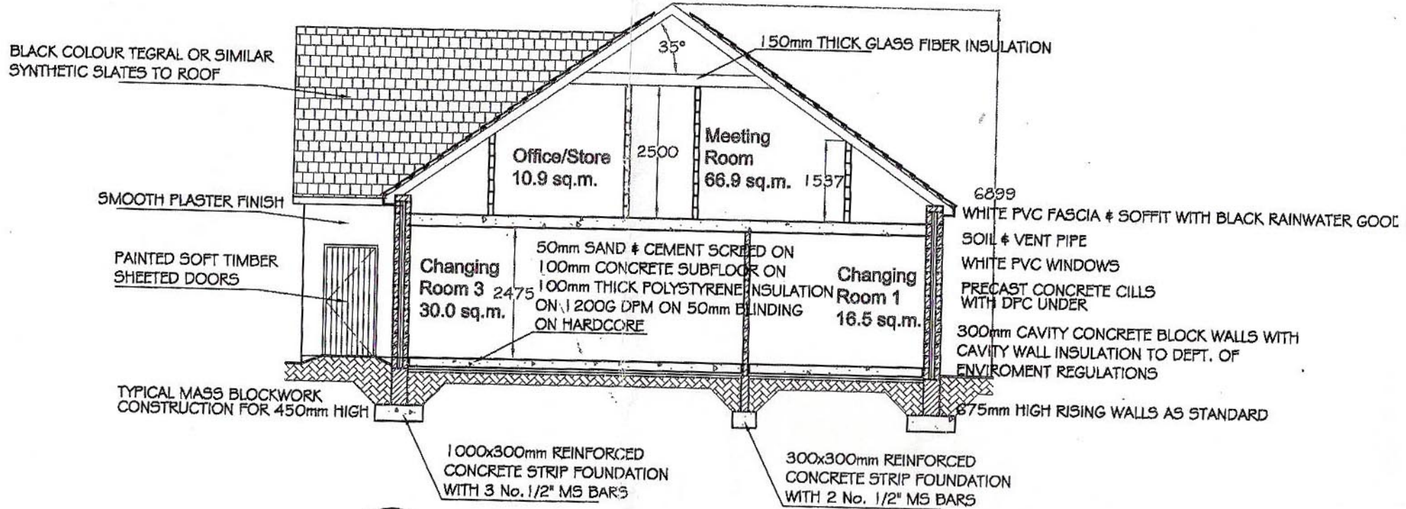
8 Section 'A-A' Thru Clubhouse 202 Scale 1:100
